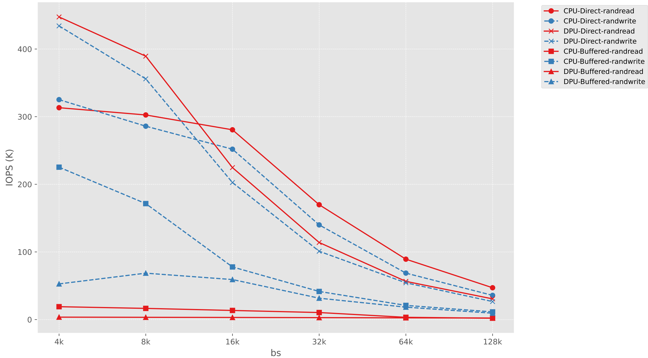
IOPS vs bs (CPU vs DPU, Direct vs Buffered)
